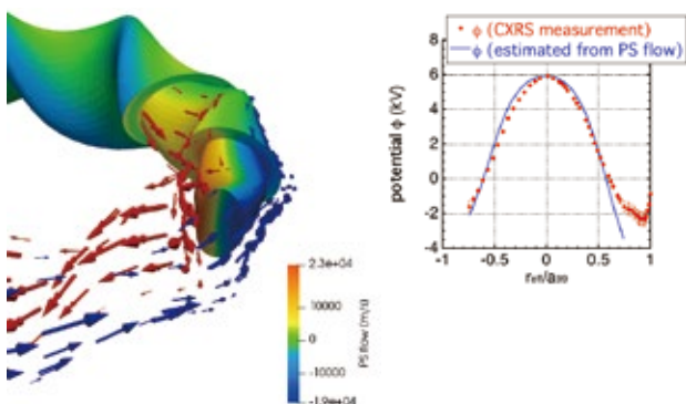
Numerical simulation of plasma flows in the magnetic confinement fusion device
