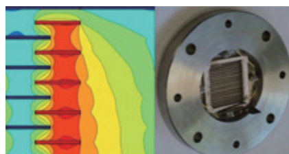
Model pump unit with no moving parts driven by the thermally driven flow in the rarefied gas
