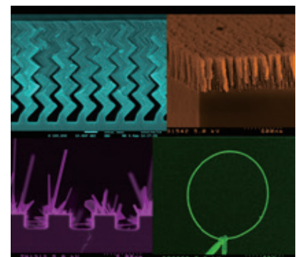
Examples of nanomorphology tailored by oblique angle deposition technique
