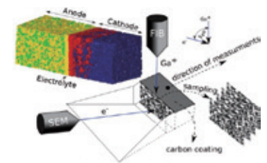
3D reconstruction of a solid oxide fuel cell microstructure
