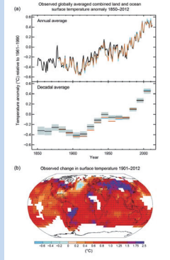
Figure SPM. 1: Observed annual and decadal global mean surface temperature anomalies from 1850 to 2012 and map of the observed surface temperature change from 1901 to 2012.
