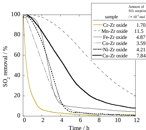
Figure 1. SO 2 removal by M-Zr oxide (M = Cr, Mn, Fe, Co, Ni, Cu, M/Zr = 1). Reaction conditions: 1000 ppm SO 2 , 10% O 2 , He balance; T = 200 °C; W/F = 1.0 g s cm -3 . The samples were calcined at 450 °C in air.
